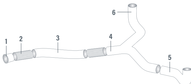
1- SES016 4- SES053 2- FLEXIBLE 5- SES007 / SES005 3- SES018 6- SES006 / SES004
