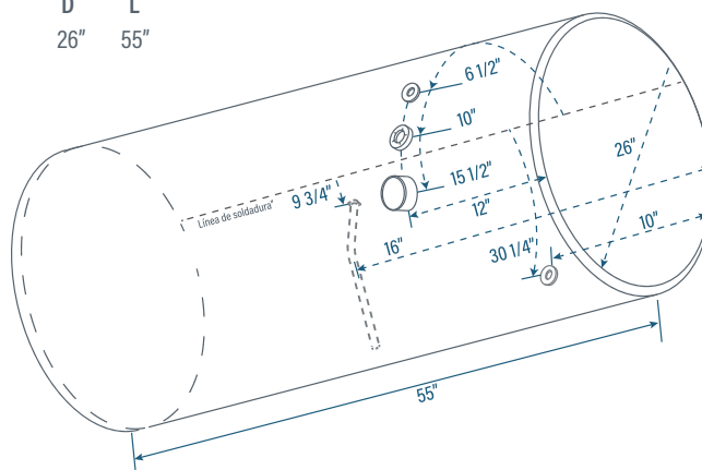
RH LH TANV47D TANV47I Volvo 1 G
